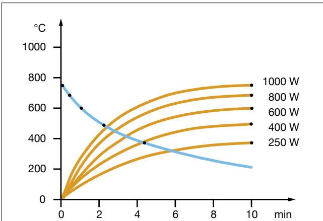
Fig. 12: Radiator temperatures Heating-up: red curves Cooling-down: blue curve
